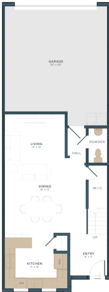
MAIN LEVEL
